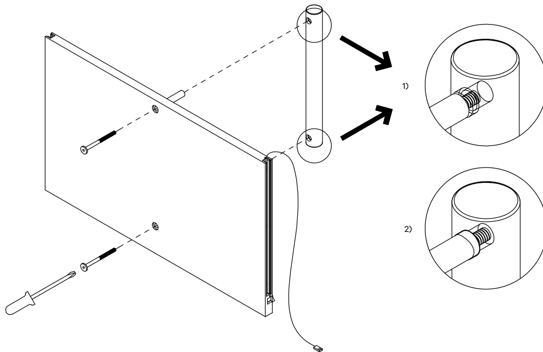
3 To avoid misalignment, first, screw both screws halfway in and only then screw them all the way in.
